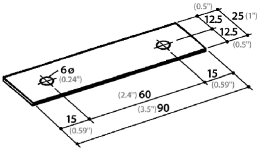
Figure 4 Backer Plate
