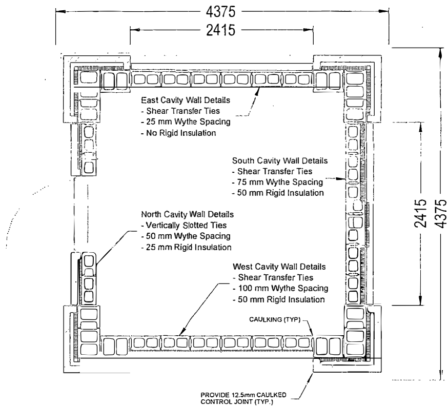
Figure 2 - Cross Section of Instrumented Region of Tower (Elev. 0 - 12040 mm)
