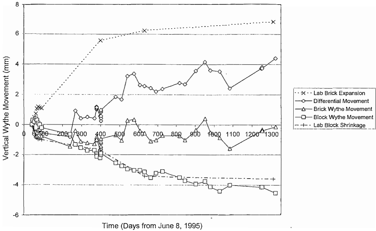
Figure 8 -South Cavity Wall Wythe Movement with Thermal Movements Removed (Cavity wall details: Shear transfer ties, 75 mm wythe spacing, 50 mm rigid insulation)
