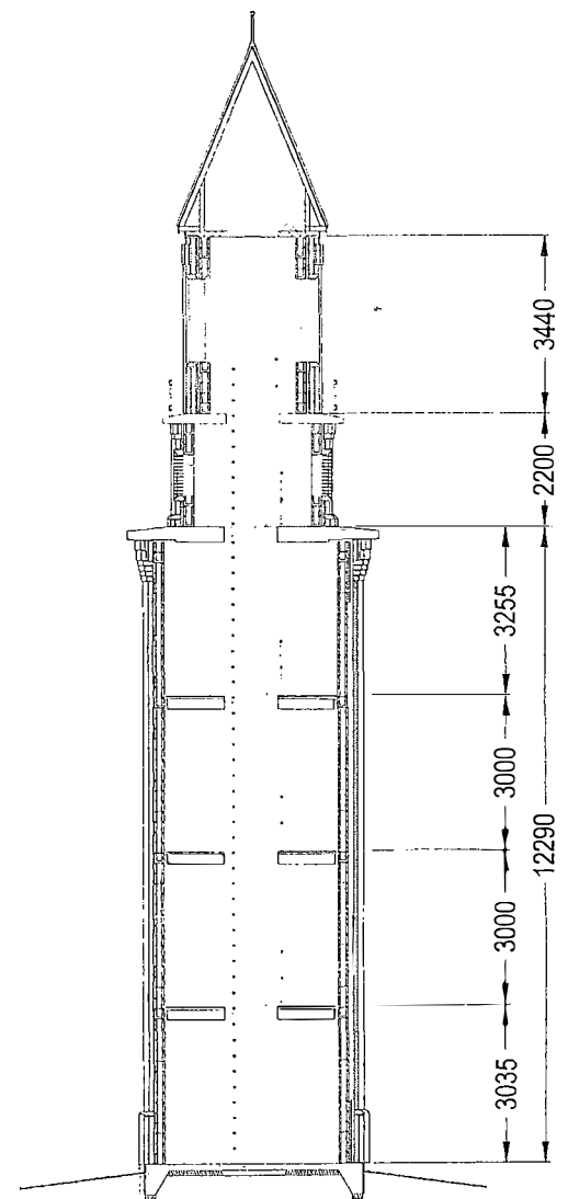
Figure 1 - Elevation of Perron Clock Tower
