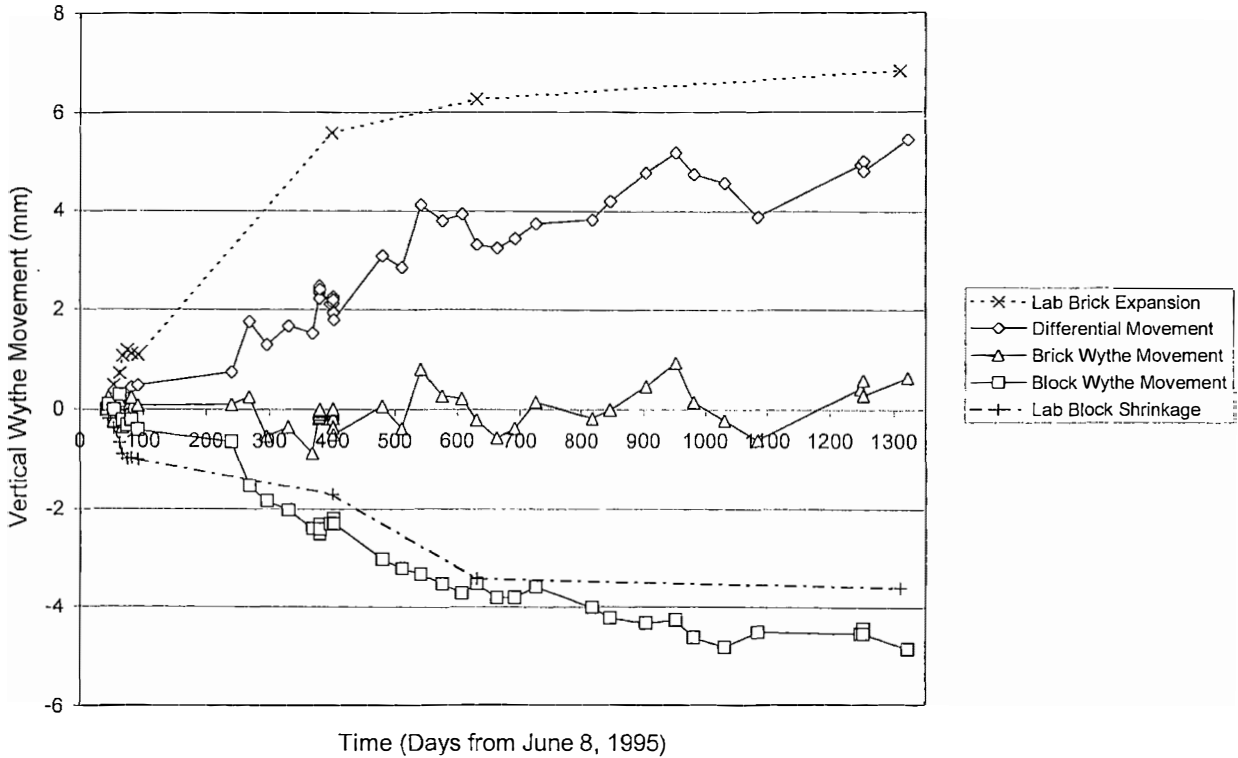
Figure 9 -West Cavity Wall Wythe Movement with Thermal Movements Removed (Cavity wall details: Shear transfer ties, 100 mm wythe spacing, 50 mm rigid insulation)
