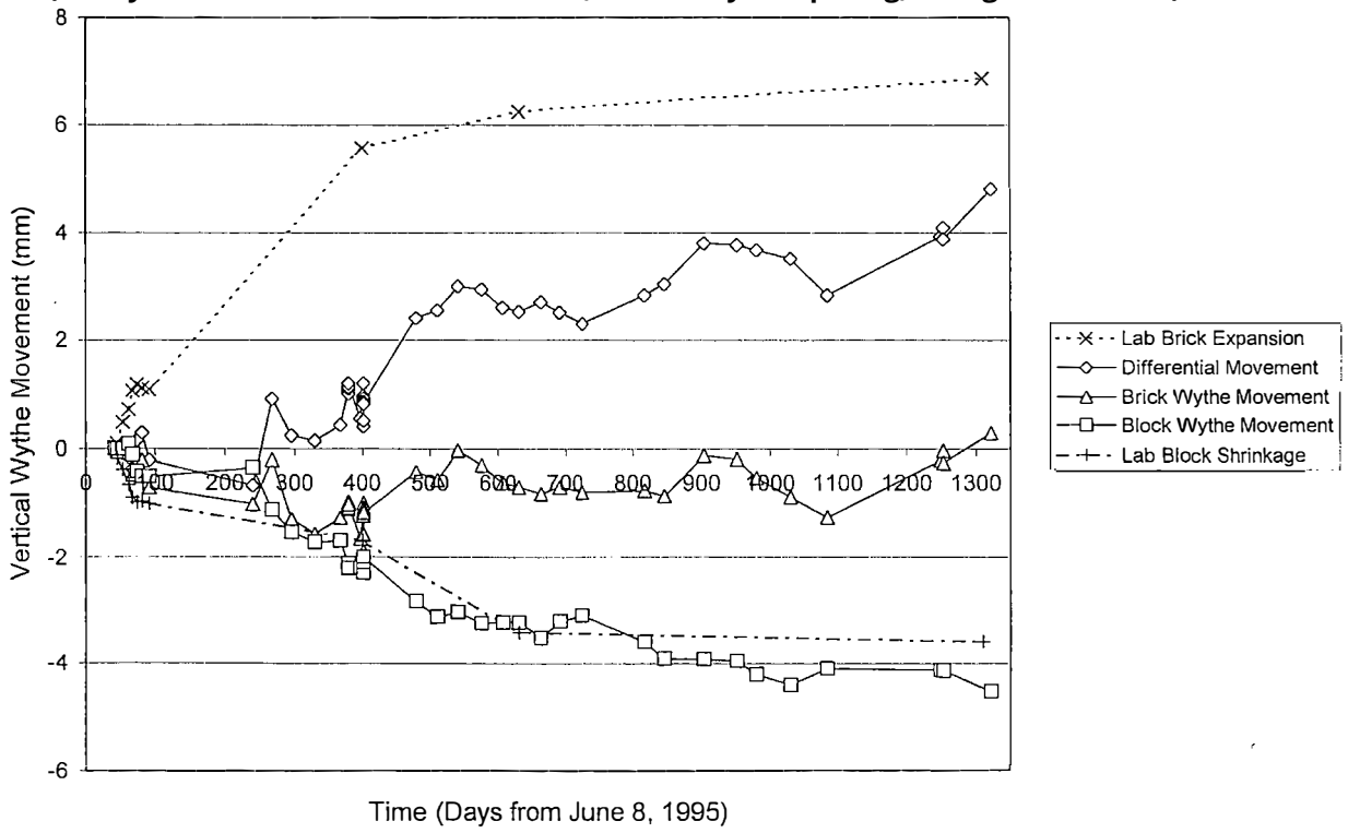
Figure 7 - East Cavity Wall Wythe Movement with Thermal Movements Removed (Cavity wall details: Shear transfer ties, 25 mm wythe spacing, no rigid insulation)
