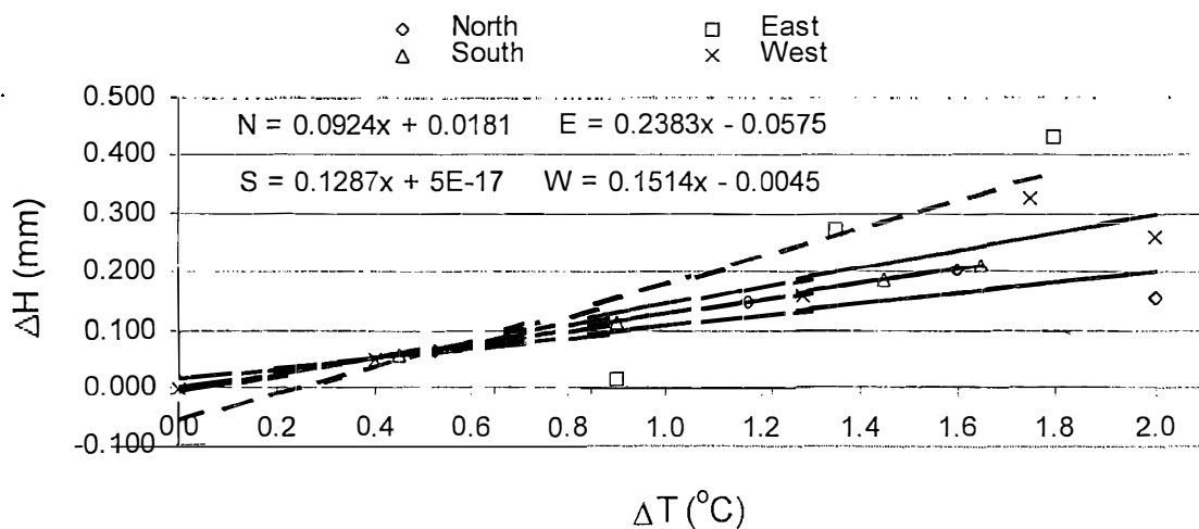
Figure 5b - Thermal Block Wythe Movement on 14 July 1996
