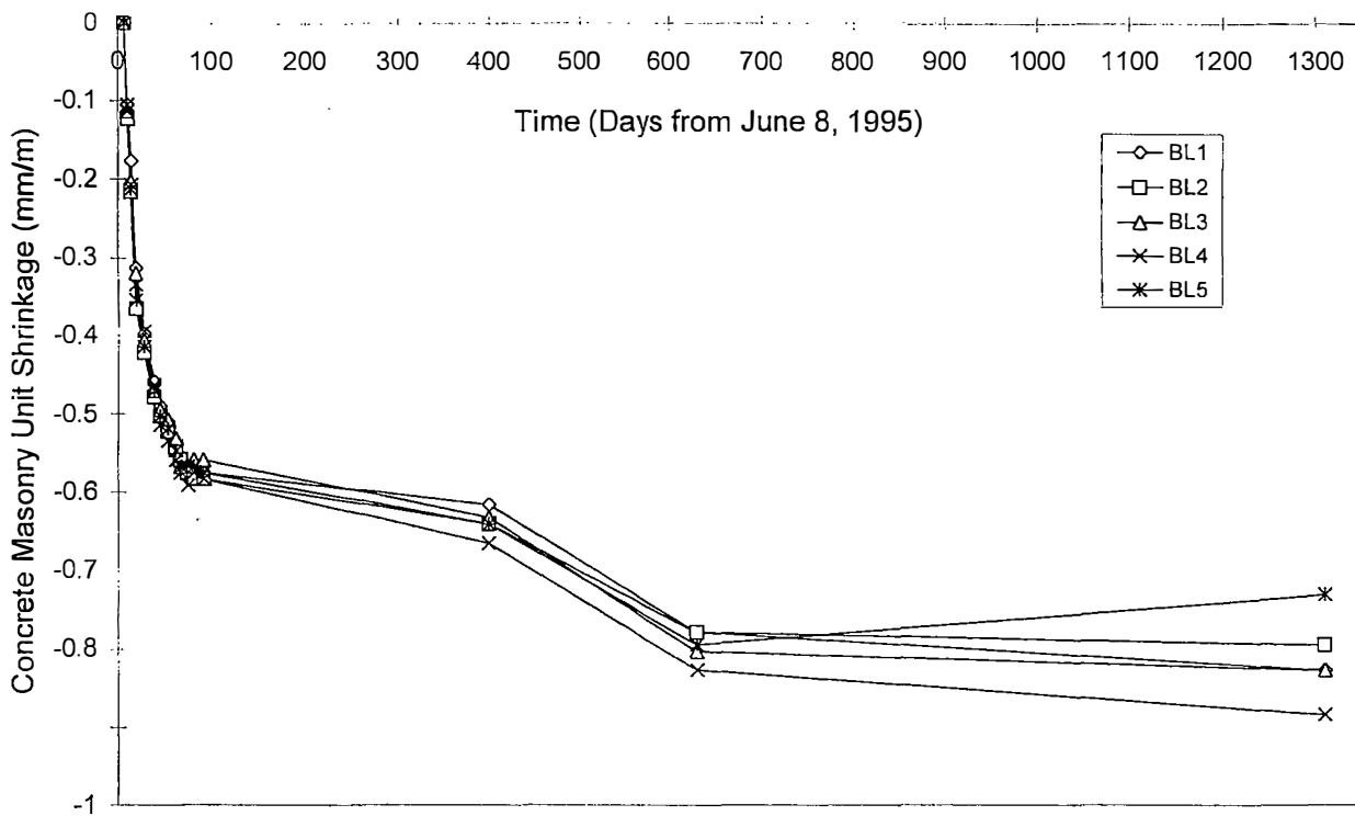
Figure 3 - Laboratory Concrete Block Movement
