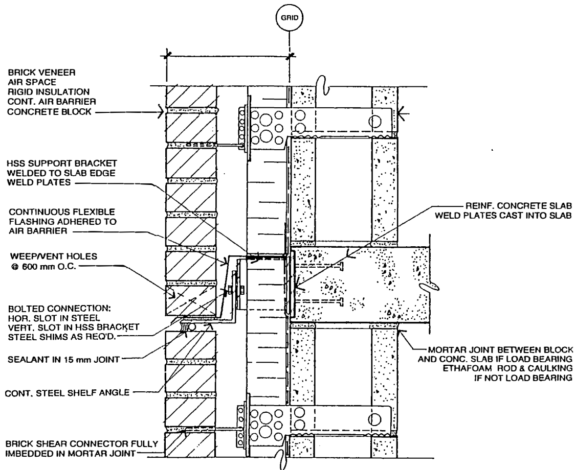
Figure 2. Brick Veneer/Concrete Block Detail At Slab Edge
