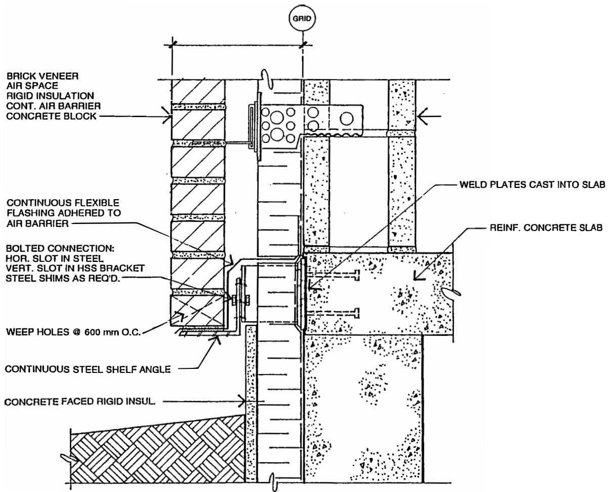
Figure 5. Brick Veneer/Concrete Block Detail At Foundation
