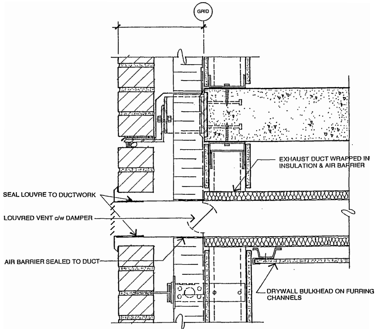
Figure 6. Brick Veneer/Steel Stud Exhaust Vent Detail
