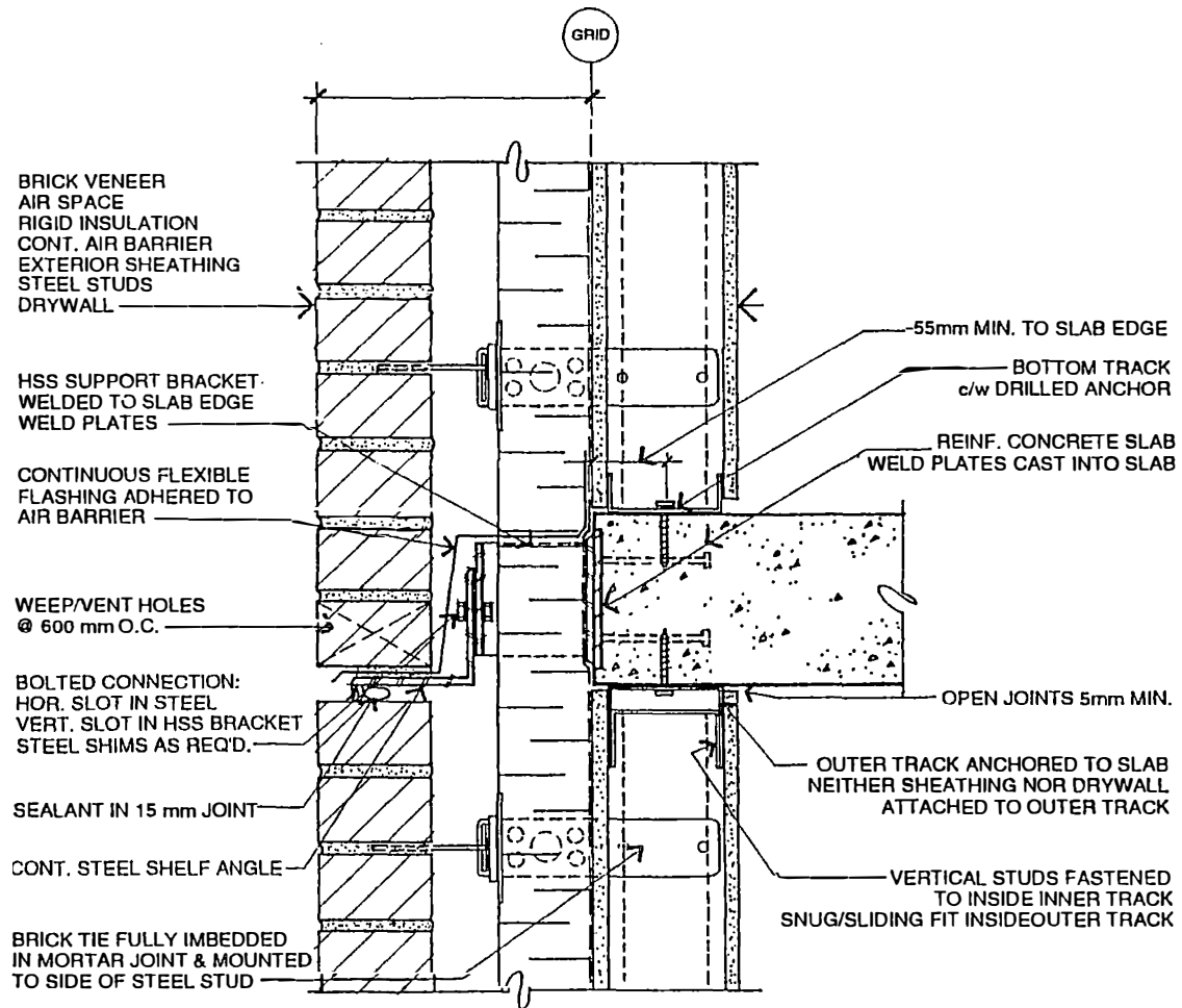
Figure 1. Brick Veneer/Steel Stud Detail At Slab Edge
